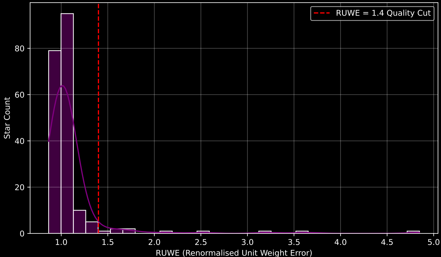
GAPOGEE DR17 Field [158+04] RUWE Distribution (n= 199)
