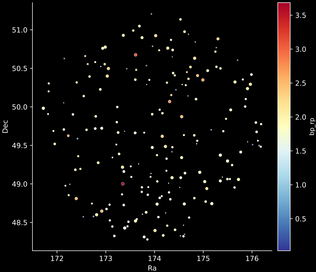
APOGEE DR17 Field: [158+04] Stars: 200
