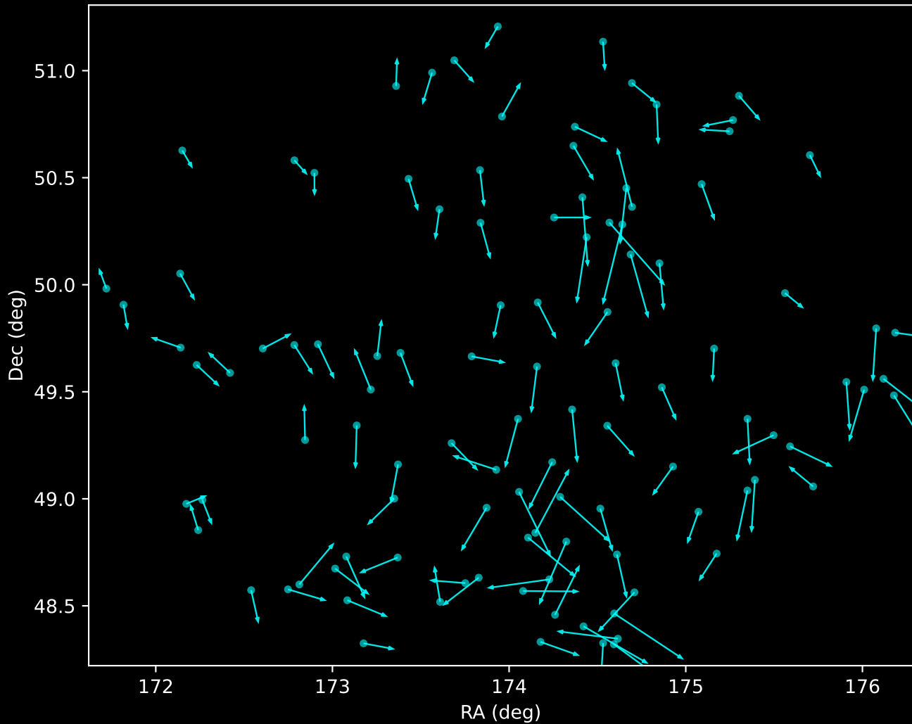
APOGEE DR17 Noise Stream Proper Motion Vectors (n=109)
