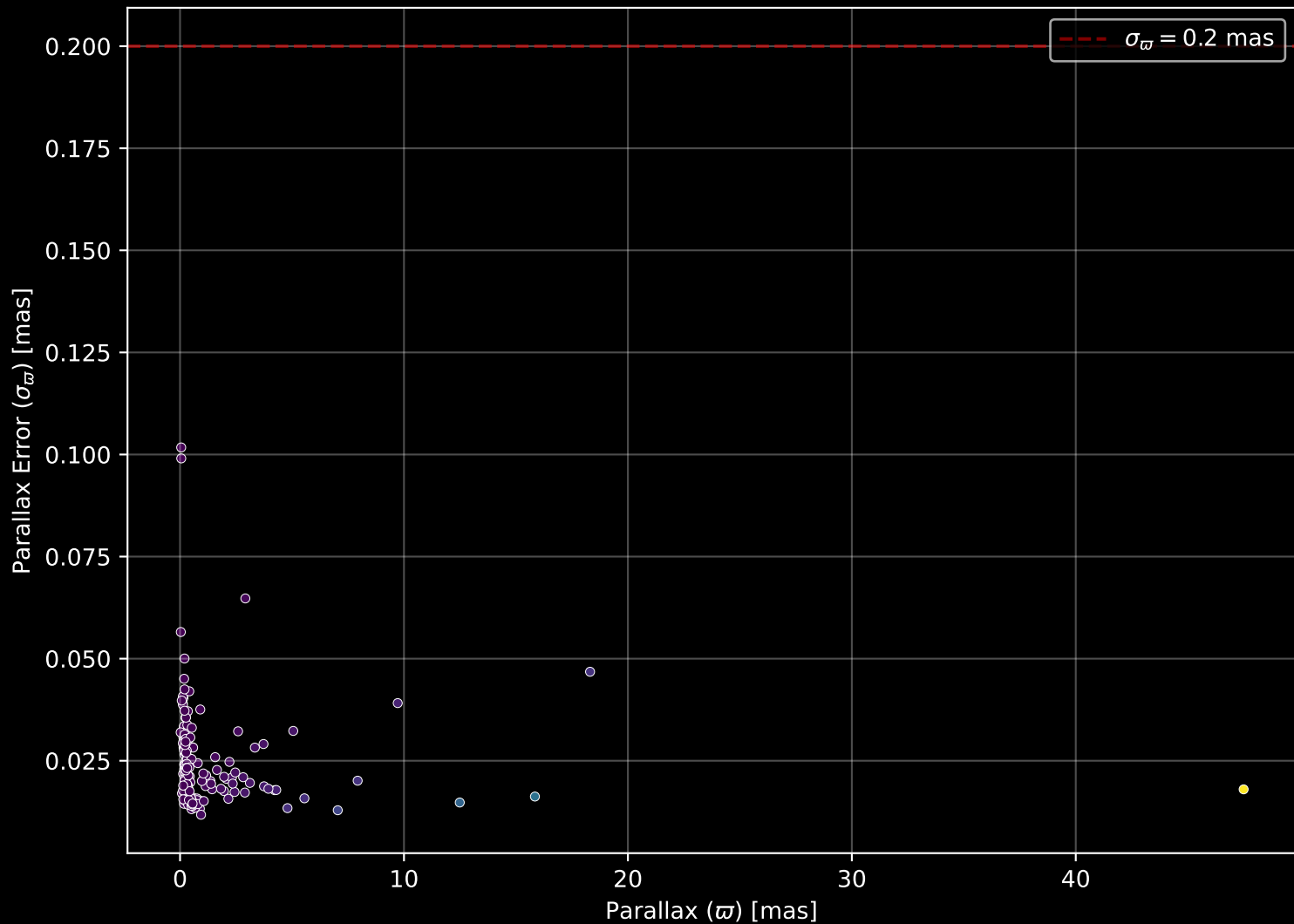
APOGEE DR17 Field: [158+04] Parallax Quality (n= 200)
