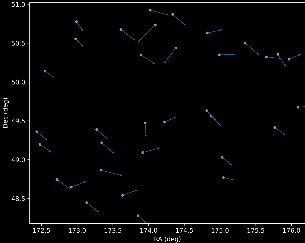
APOGEE DR17 Cluster 0 Proper Motion Vectors (n=34)
