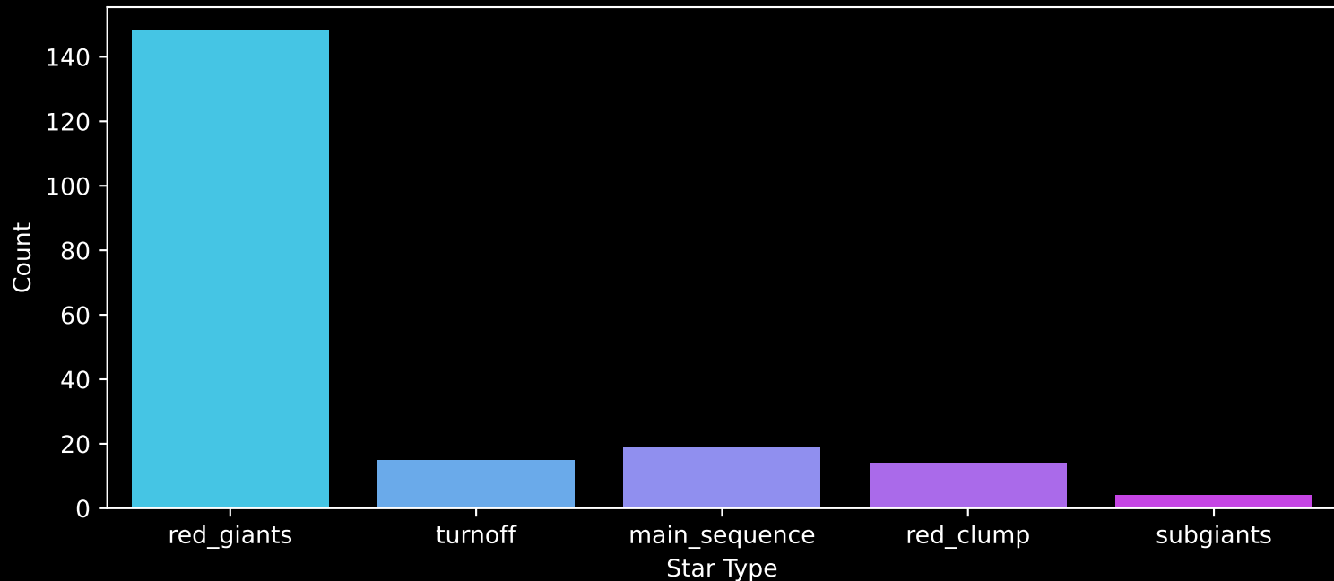
APOGEE DR17 Field: [158+04] Count plot of Star Type
