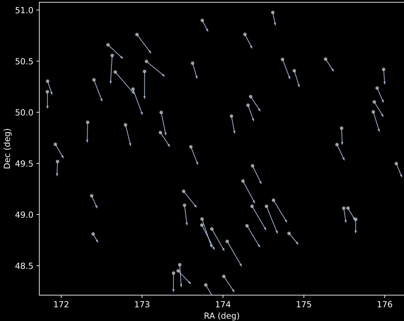
APOGEE DR17 Cluster 1 Proper Motion Vectors (n=57)
