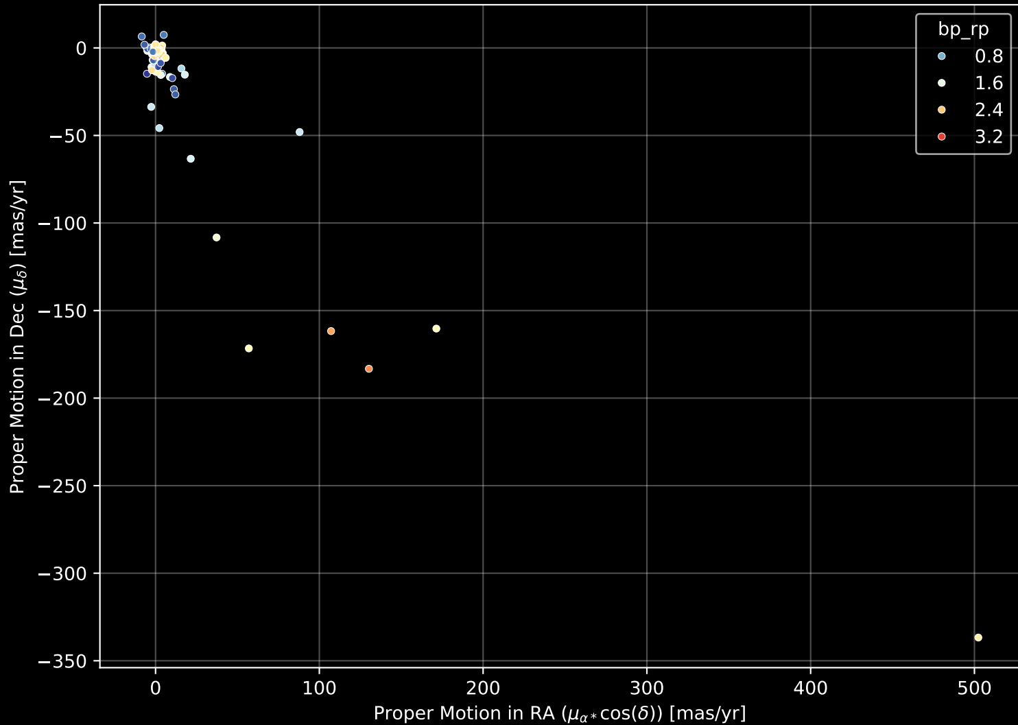
APOGEE DR17 Field: [158+04] Proper Motion Diagram (n= 200)
