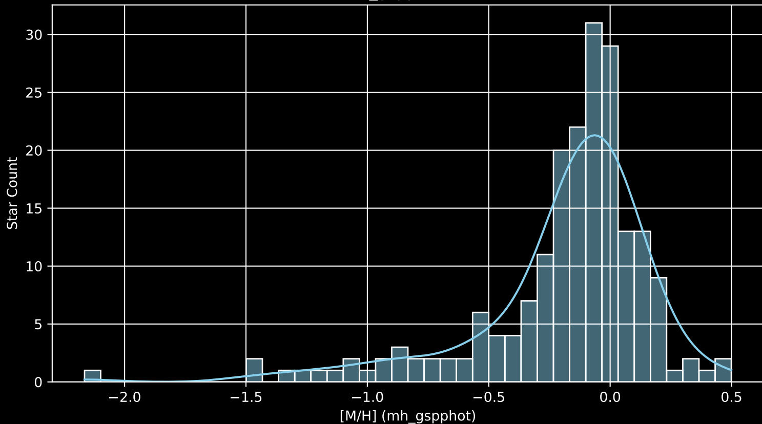
APOGEE DR17 Field: [158+04 [M/H] (mh_gspphot) (n= 198)
